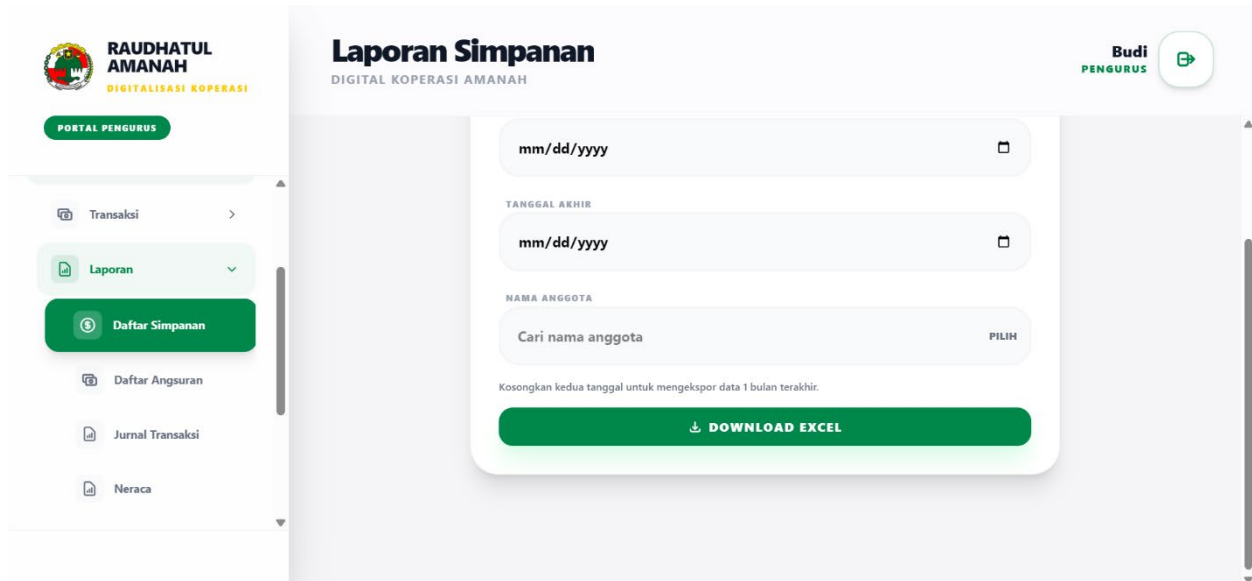
Figure 15 Reporting
