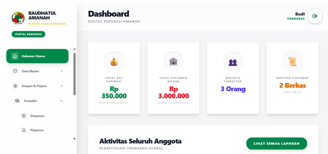
Figure 9 Administrator Dashboard
