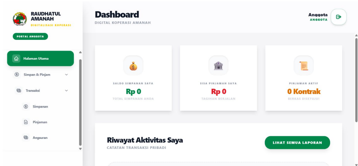
Figure 10 Member Dashboard
