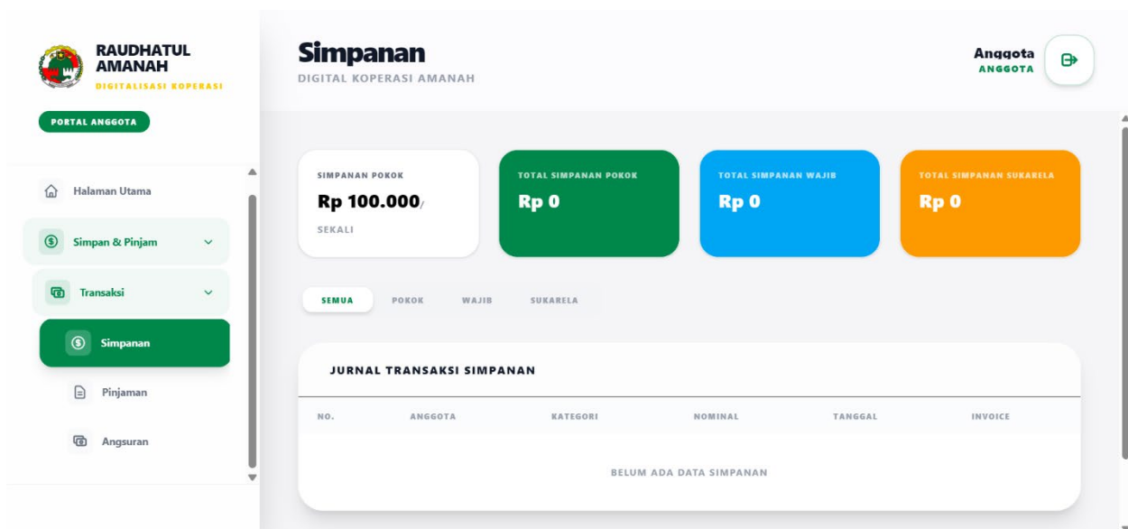
Figure 11 Saving Management
