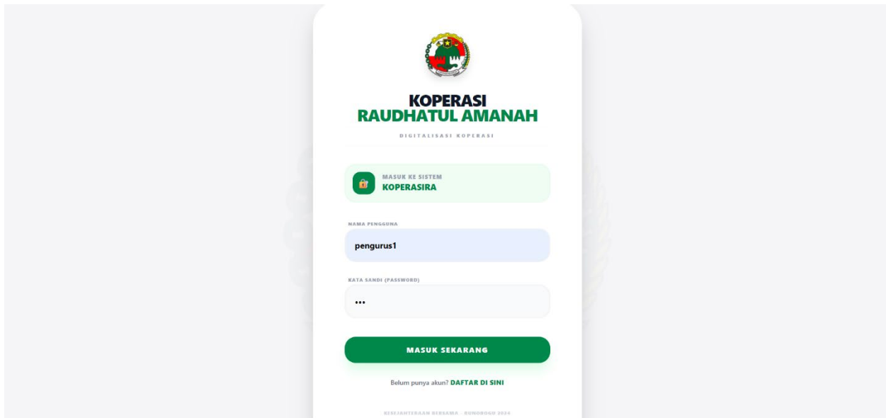
Figure 8 Login Interface
